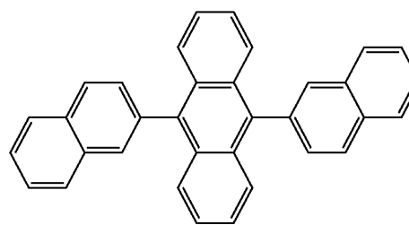
DNA
